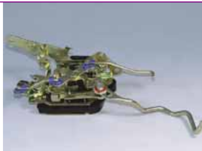
CW-DL-0653 TOYOTA RZH 104 DOOR LOCK ASSY FL 69320-95J06
