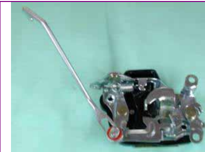
CW-DL-0619 TOYOTA HILUX RN55 '84-88 DOOR LOCK ASSY FL 69320-89109
