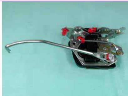
CW-DL-0620 TOYOTA HILUX YN55 '84-88 DOOR LOCK ASSY RR 69330-89103
