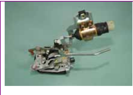
CW-DL-0573 SUZUKI ESCUDO -99 DOOR LOCK ASSY FR 82201-62A00
