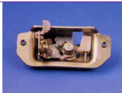
CW-DL-0411 MISUBISHI MINICAB 800 VARICA 1100CC TRUNK LID LOCK ASSY MB331428
