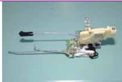
CW-DL-0180 HINO 10.5-15 (17) T21-35T '03-04 DOOR LOCK ASSY FR 69410-2052 69310-E0080
